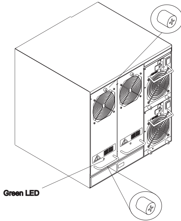
Figure 1 Fan Tray Captive Screws
