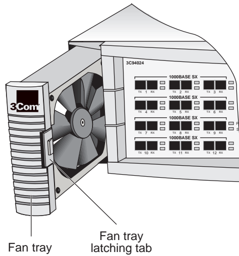
Figure 2 Fan Tray Assembly Removal and Replacement: CoreBuilder 9400
