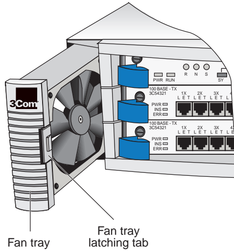
Figure 1 Fan Tray Assembly Removal and Replacement: CoreBuilder 3500
