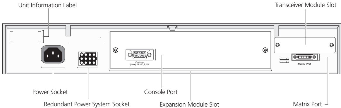
Figure 3 VCN Services Switch 10 - Rear View
